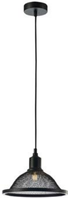
69818 Indoor | Lámpara Colgante Malla Negro | Black Metal | Use/Utiliza: E27 1 Pc (Not Include) | Size/Medida (H / W / D) (mm) D250*H180
